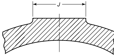
Figure 4 Bosses for Auxiliary Connections
