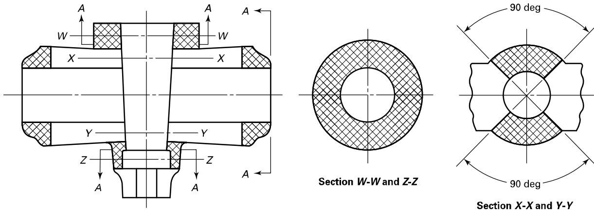
Figure 14 Plug Body
