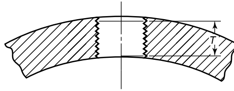
Figure 3 Thread Length for Auxiliary Connections
