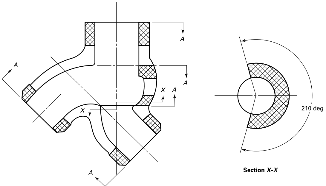
Figure 10 Elbow Down (Pressure Seal Bonnet)
