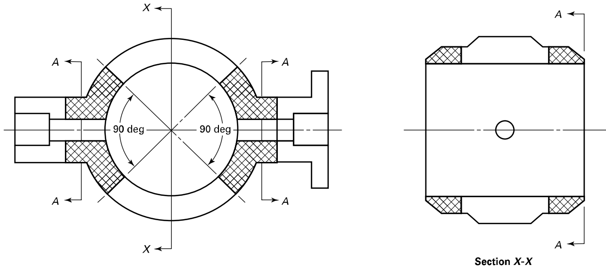
Figure 13 Butterfly Body
