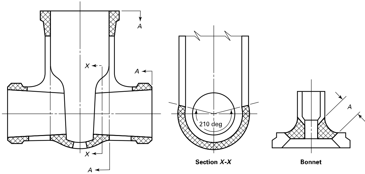
Figure 7 Gate Body (Pressure Seal Bonnet)
