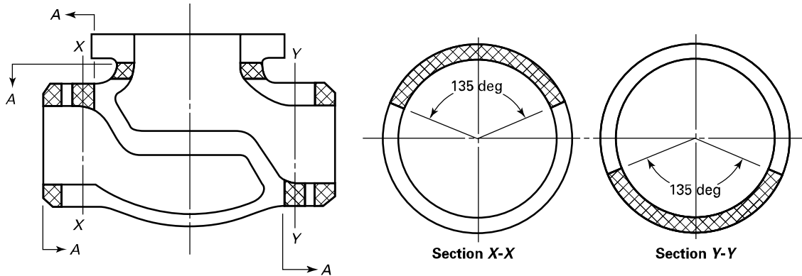
Figure 12 Globe Body (Flanged Bonnet)
